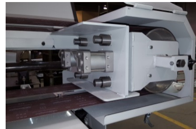
Pneumatic Belt Tensioner
