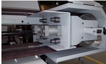
Pneumatic Belt Tensioner
