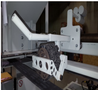
Contact Wheel
