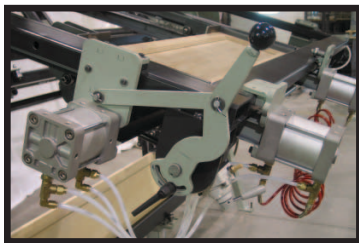
GAS SPRING ASSISTED LEVER
