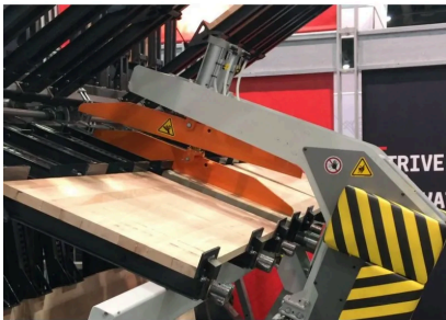
DOUBLE ACTUATED FLATTENER
