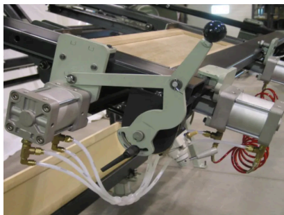
SINGLE LEVER FOR EASY MOVEMENT OF THE HORIZONTAL CLAMP
